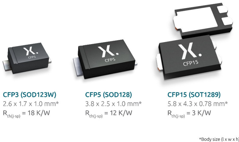
Figure 5: Nexperia Trench Schottky rectifiers in clip-bonded FlatPower packages
