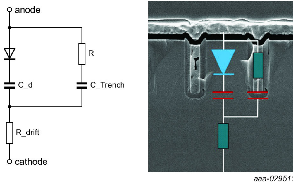
Figure 3: Equivalent circuit diagram of a Trench Schottky rectifier. The circuit elements are highlighted in the device cross section.
