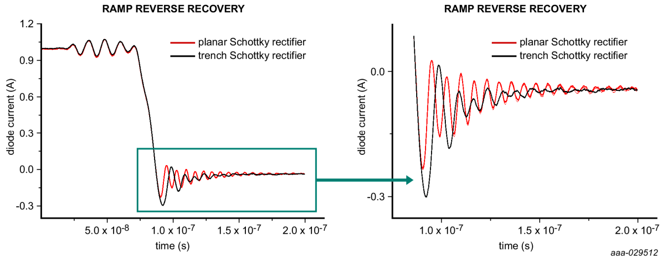
Figure 4: Ramp reverse recovery measurements on Trench and planar rectifiers. 100A/ \mu s ramp.
